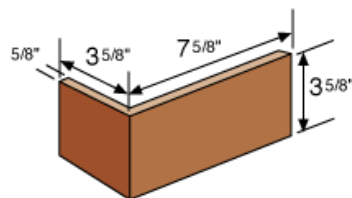
3 5/8" x 7 5/8" CLOSURE CORNER
