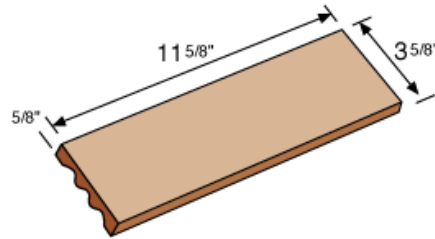
3 5/8" x 11 5/8" UTILITY
