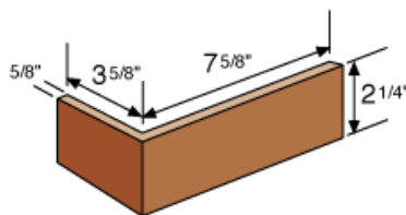
2 1/4" x 7 5/8" MODULAR CORNER
