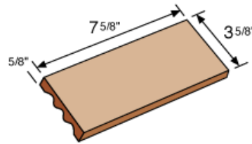
3 5/8" x 7 5/8" CLOSURE
